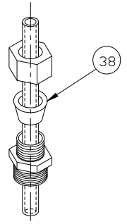
INJECTION FITTING
