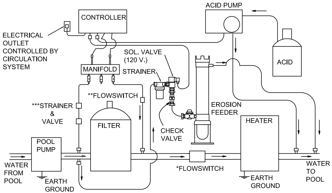
SYSTEM USING EROSION FEEDER WITH ACID PUMP (CALCIUM HYPOCHLORITE & MURIATIC ACID)
