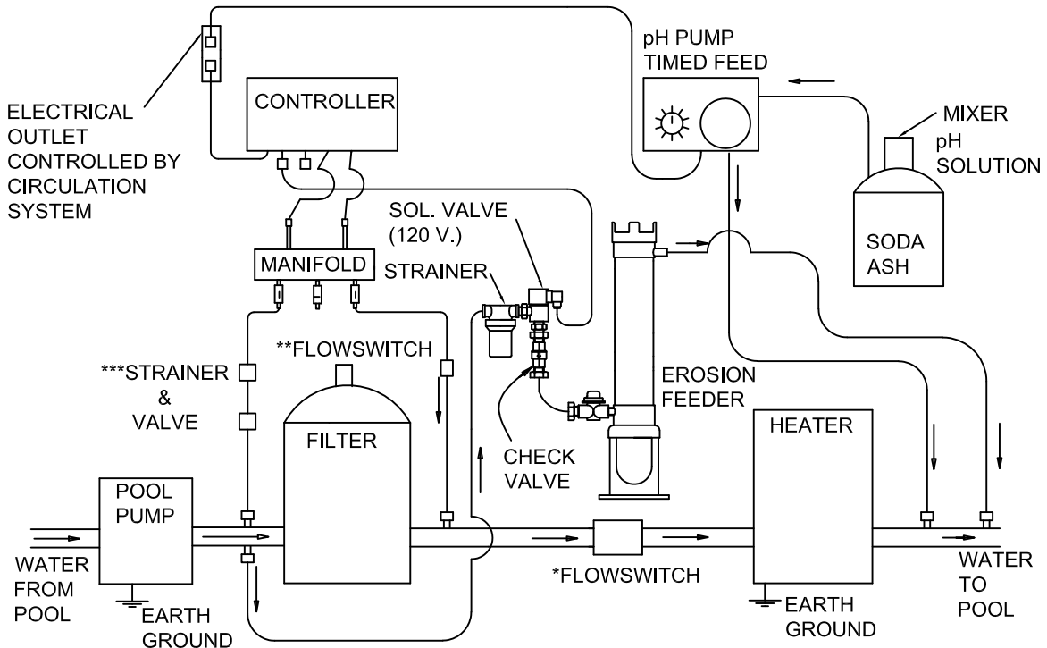
SYSTEM USING EROSION FEEDER (TRI-CHLOR/ DI-CHLOR) WITH SODA ASH PUMP
